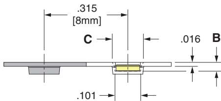
Series 1593 (Tape Pocket Details)
