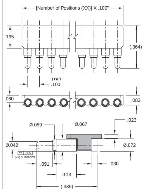
Series 810 Single Row
