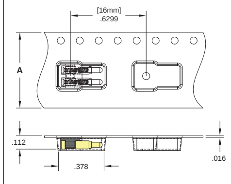
Series 810 (Tape Pocket Details)
