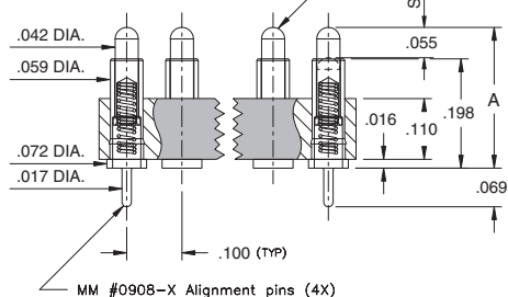
MM #0908-X Alignment pins (4X)
