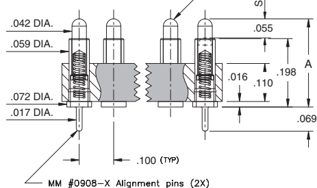
MM #0908-X Alignment pins (2X)
