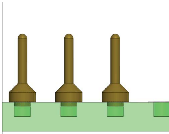
Figure 3: MM 0508 Soldered Into Blind Via Holes on PCB
