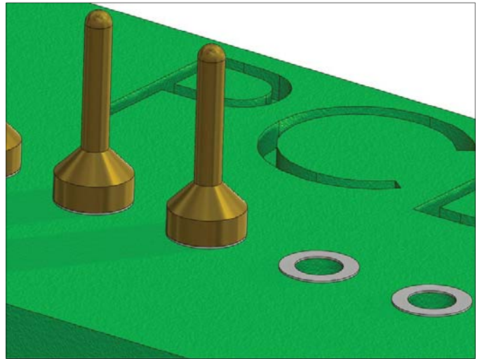
Figure 2: MM 0508 Soldered Into Blind Via Holes on PCB
