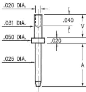
311X-X-00-XX-00-00-08-0 Swage mount in .035 mounting hole
