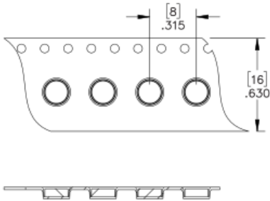
1656-X-57 Tape & Reel Details
