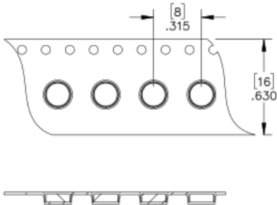
1656-X-57 Tape & Reel Details
