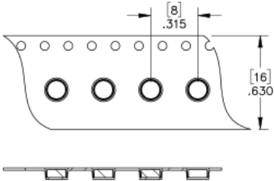
1625-X-57 Tape & Reel Details
