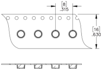
1618-X-57 Tape & Reel Details
