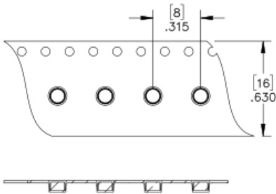
1593-X-57 Tape & Reel Details
