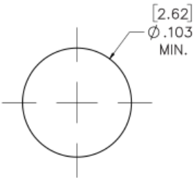
Suggested P.C.B. Footprint
