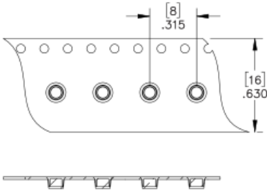
1578-X-57 Tape & Reel Details
