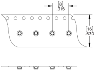
1559-X-57 Tape & Reel Details
