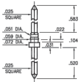
1221-0-05-XX-00-00-01-0 Press-fit in .056 mounting hole
