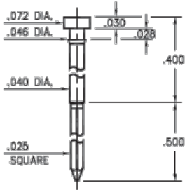
1215-3-05-XX-00-00-01-0 Press-fit in .043 mounting hole
