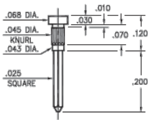
1124-0-05-XX-00-00-01-0 Press-fit in .043 mounting hole
