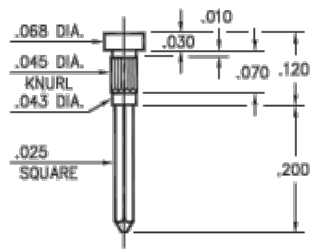
1124-0-05-XX-00-00-01-0 Press-fit in .043 mounting hole
