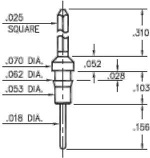
1083-0-05-XX-00-00-01-0 Press-fit in .059 mounting hole
