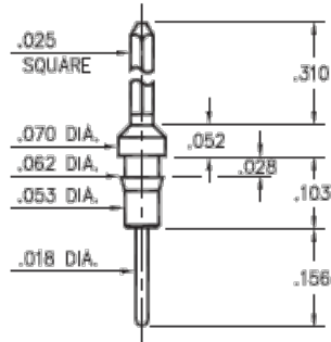
1083-0-05-XX-00-00-01-0 Press-fit in .059 mounting hole
