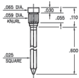
1094-0-05-XX-00-00-01-0 Press-fit in .056 mounting hole
