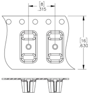
5058-0-57 Tape & Reel Details
