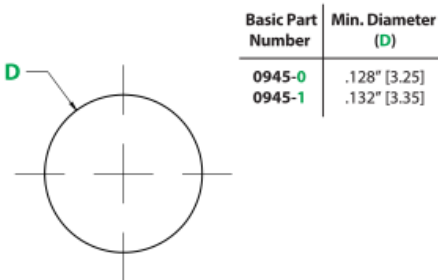
Suggested P.C.B. Footprint
