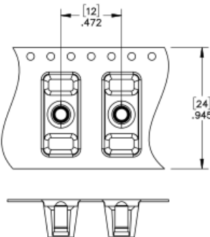
0945-0-57 Tape & Reel Details
