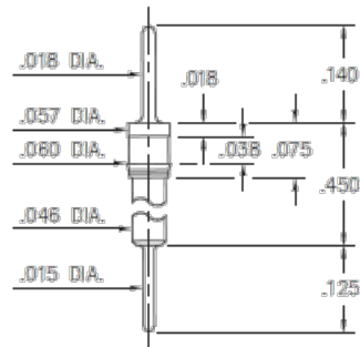
8885-0-00-XX-00-00-03-0 Press-fit in .057 mounting hole
