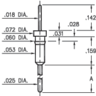
3409-X-00-XX-00-00-03-0 Press-fit in .057 mounting hole
